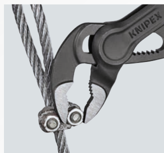
Amazing flexibility: The self-locking effect of the KNIPEX Cobra® XS enables it to grip round materials up to Ø 28 mm extremely reliably – and, due to its very slim head, it can also hold small components in place.
